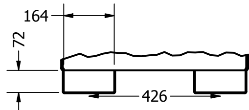
DETAIL A SCALE 1 / 12
